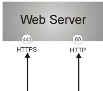
Figure 87 HTTP/HTTPS Implementation
